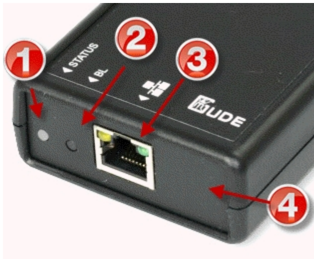
Anschlüsse an der Expert Sensor Box 7211
